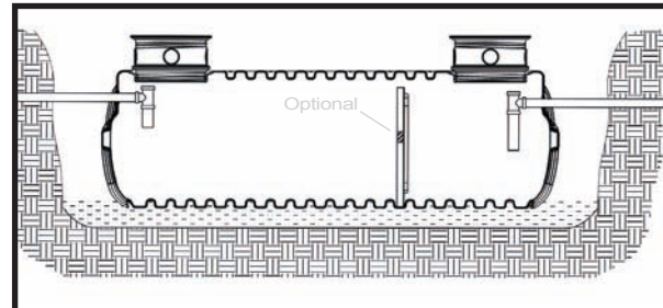
FIG.3 Plumbing Install
