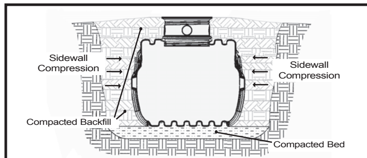
FIG.4 Backfilling
